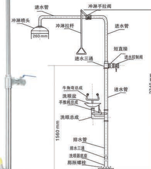
◎BTF41 紧急冲淋洗眼器 (手动排空防冻型) BTF41 emergency shower & eye washer (manual empty & anti-freeze)
