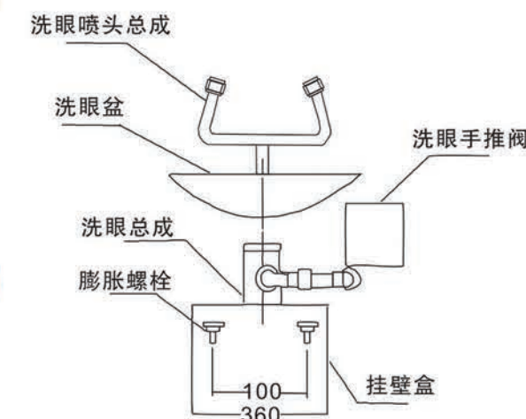
◎BTG11-A 双防不锈钢挂壁式紧急洗眼器 (ABS防腐涂层) BTG11-A Double protection stainless steel emergency eye wash(ABS anti-corrosion coating)
