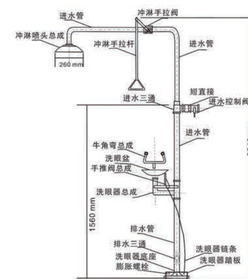
◎BTF61 紧急冲淋洗眼器 (手动排空防冻+脚踏板) BTF61 emergency shower & eye washer (manual empty & anti-freeze+pedal)
