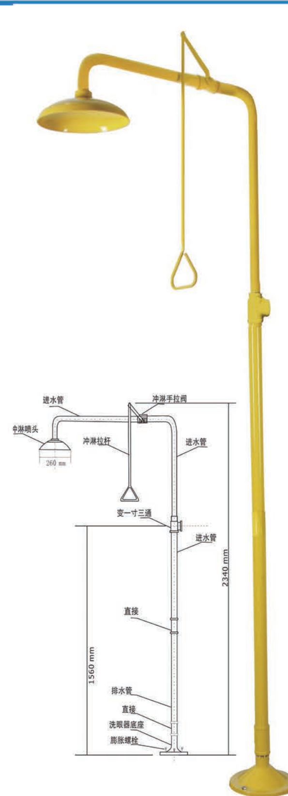
◎BTLC11-A 落地式紧急冲淋器 BTLC11-A Vertical emergency shower
